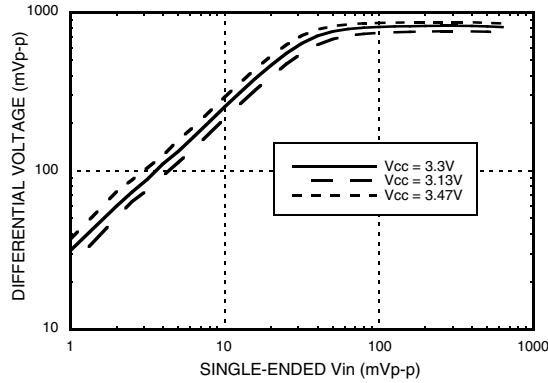
Differential Output vs. Vinup & Supply Voltage @ 16 GHz [1]
