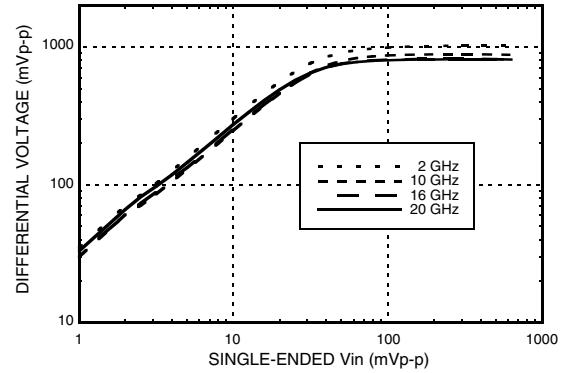
Differential Output vs. Vinup & Frequency [1][2]
